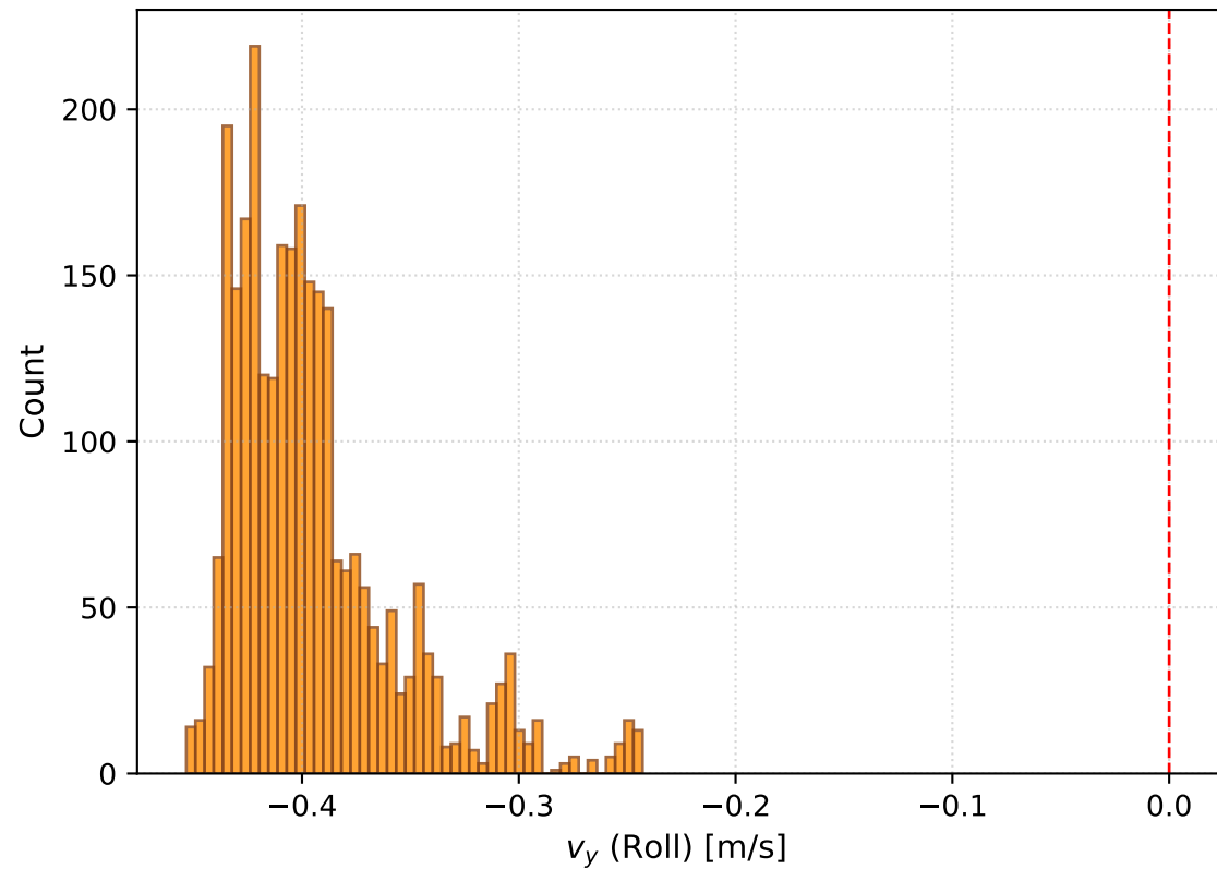
Roll Velocity Commands ( \sigma=0.0389 m/s)
