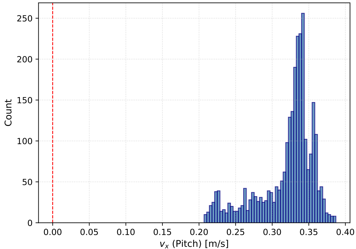
Pitch Velocity Commands ( \sigma=0.0386 m/s)
